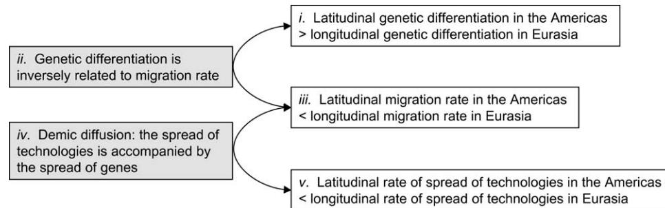
Fig. 1. The connection between spatial patterns of genetic variation and the spread of technologies. The figure illustrates that conditional on (ii) and (iv), a test of (i) provides a test of (v). This line of reasoning suggests a genetic approach to testing the argument that continental axes of orientation explain relative differences in the spread of technologies in Eurasia and the Americas.
