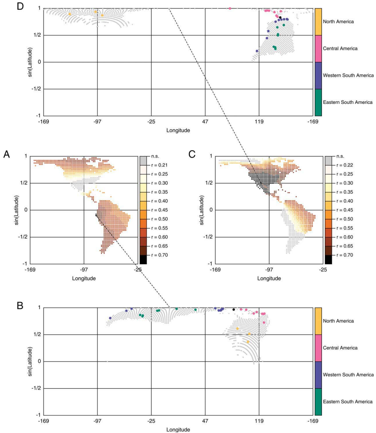
Fig. 5. Relationship of genetic distance and latitudinal and longitudinal distance based on rotated coordinates in the Americas. A: Partial Mantel correlations between F_{ST} and rotated latitudinal distance with waypoints, controlling for mean heterozygosity, at 1,246 poles in the Americas. The color of a point corresponds to the partial Mantel correlation r when population locations in Eurasia are rotated about that point. The range of r values significantly different from zero at the 5% level is [0.2191, 0.7094]; 91.7% of poles produced significant partial Mantel test results (among 10^4 permutations). The model shown had the highest proportion of significant partial Mantel tests of the regressions on latitudinal distance after rotating about poles in the Americas. B: Rotation of American population locations about the pole ( 5.73917^\circ \text{ S}, 80.8^\circ \text{ W} ), plotted here with \psi_0 = 90^\circ . The pole is indicated by an open circle in (A) from which a dashed line is drawn to (B) at ( 90^\circ \text{ N}, 0^\circ \text{ E} ). The partial correlation between F_{ST} and latitudinal distance (controlling for mean heterozygosity) was calculated using latitudinal distance between population locations after applying the rotation. C: Partial Mantel correlations between F_{ST} and rotated longitudinal distance with waypoints, controlling for mean heterozygosity, across poles in the Americas. The range of r values significantly different from zero at the 5% level is [0.2243, 0.7468], and 79.7% of poles produced significant partial Mantel test results (among 10^4 permutations). D: Rotation of American population locations about the pole ( 30^\circ \text{ N}, 107.8^\circ \text{ W} ), plotted here with \psi_0 = -90^\circ . The pole is indicated by an open circle in (C) from which a dashed line is drawn to (D) at ( 90^\circ \text{ N}, 0^\circ \text{ E} ). Because of this pole's location near the Pima population, an angle \psi_0 that placed all populations in the same hemisphere (i.e., with maximal rotated longitudinal distance between a population pair less than 180^\circ ) could not be found.
